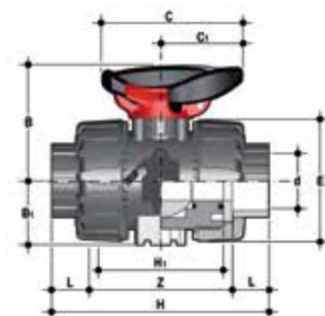
VKDIA/SHX 2-way ball valve with handle lock and STAINLESS steel threaded inserts with female ends for solvent welding, metric series
