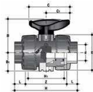
VKDIA/SHX 2-way ball valve with handle lock and STAINLESS steel threaded inserts with female ends for solvent welding, metric series
